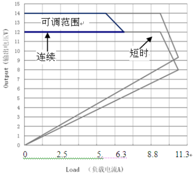
图 3-1-2 Output V-I curve (输出负载特性曲线)
