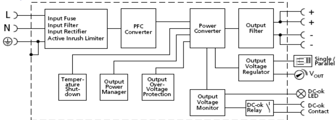
Functional diagram
